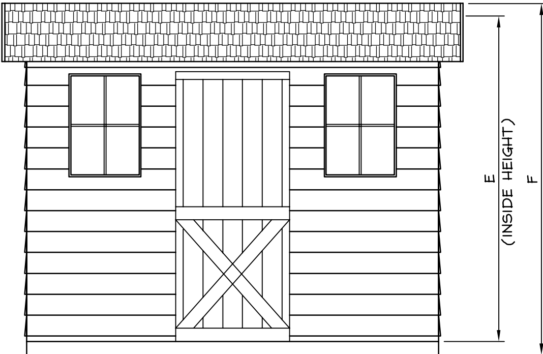
FRONT VIEW
